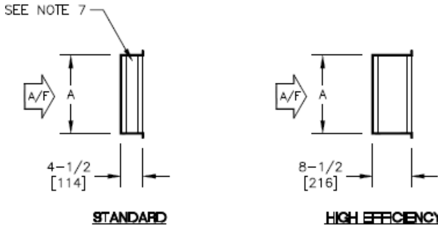
SIDE VIEWS
