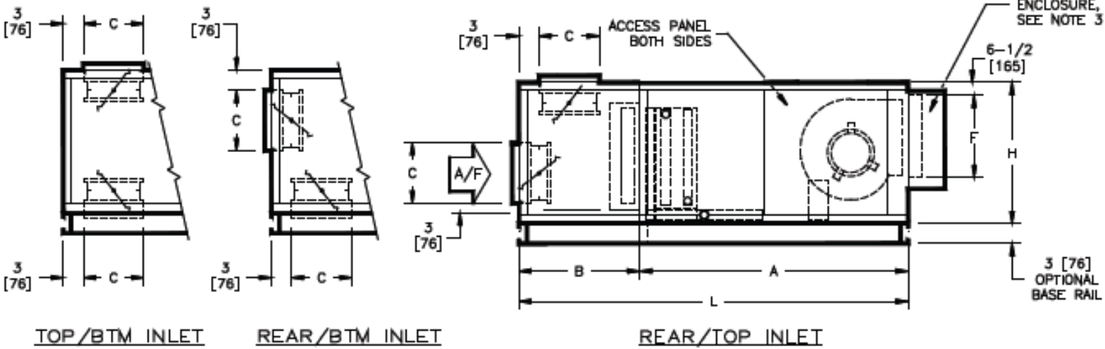
SIDE VIEW
