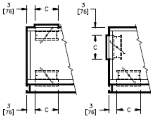
TOP/BTM INLET
