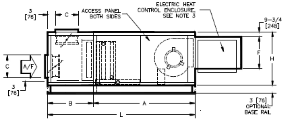
REAR/TOP INLET
