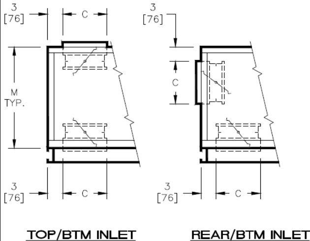
TOP/BTM INLET
